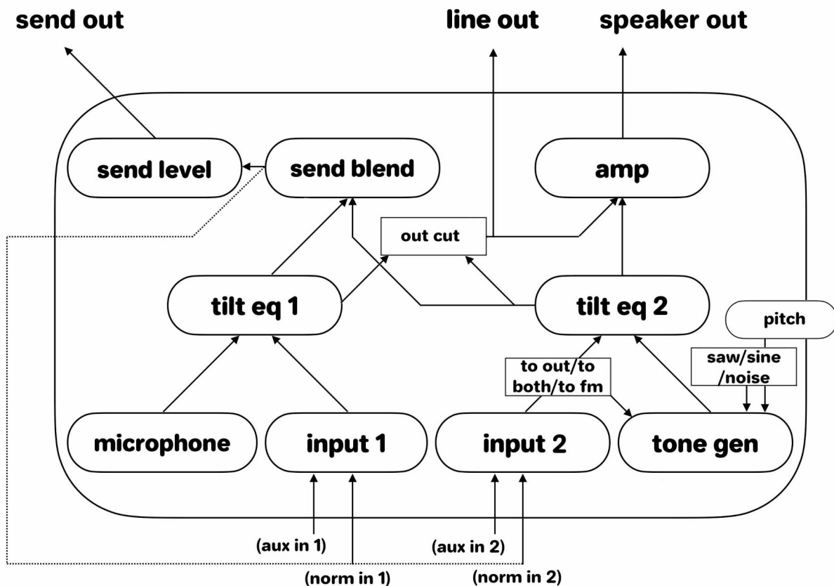
Figure 2: signal flow of the System Sound 4
